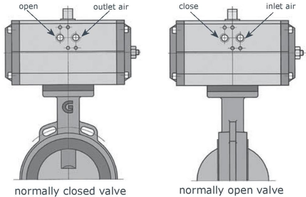
single acting actuator - 3 ways solenoid valve
